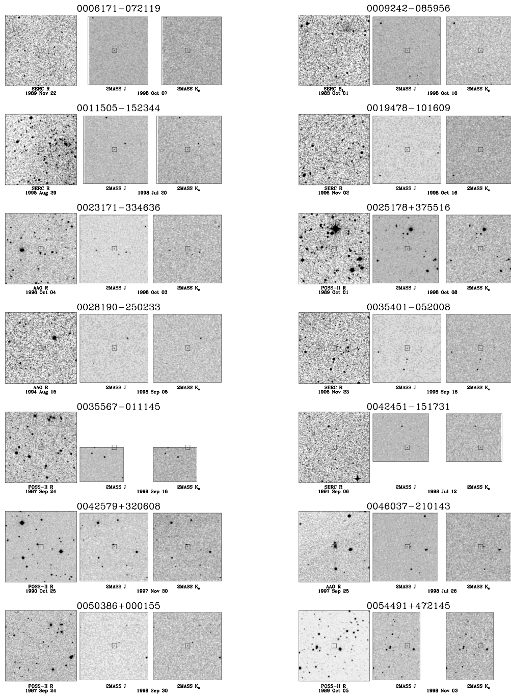
Figure A.30: DSS, XDSS, 2MASS J, and 2MASS K s images of candidates from the rdb0400 Sample. Images are nominally 5' \times 5' , oriented with North up and East to the left. Candidate positions are indicated by 20'' \times 20'' boxes.
