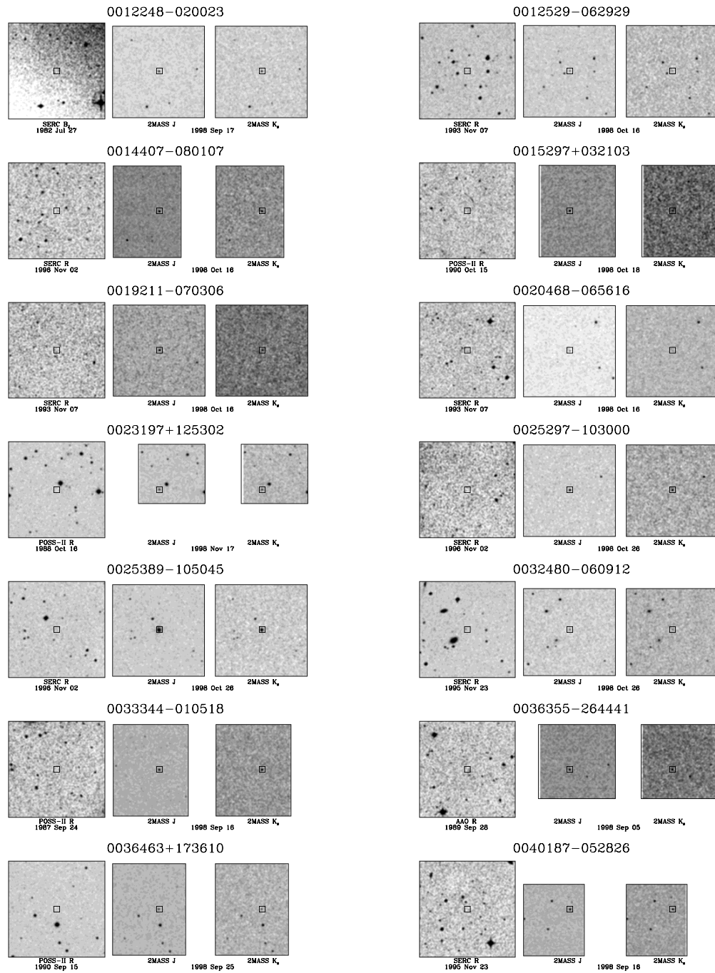
Figure A.50: DSS, XDSS, 2MASS J, and 2MASS K s images of candidates from the rdb0600 Sample. Images are nominally 5' \times 5' , oriented with North up and East to the left. Candidate positions are indicated by 20'' \times 20'' boxes.
