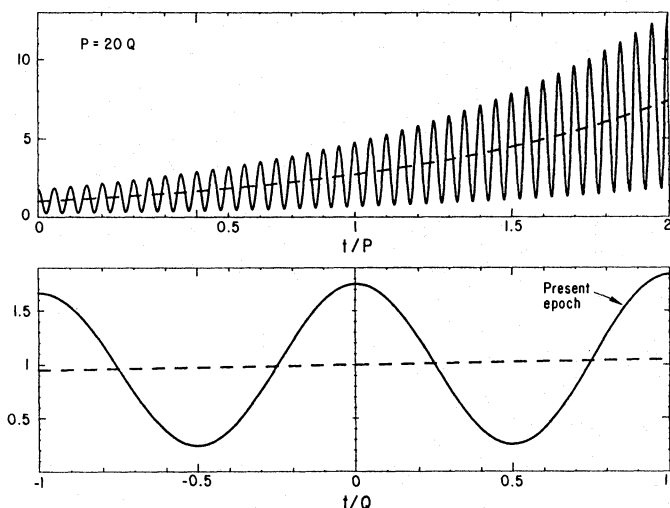
Fig. 1. S(t) plotted against t/P (upper panel) and against t/Q (lower panel).
