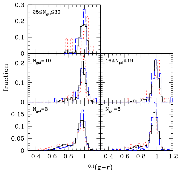
Figure 6. Distributions of g-r color of central galaxies as a function of group richness, for M_r < -19.9 . Solid black histograms show the predictions of the model (Skibba & Sheth 2008); dashed blue histograms show the measurements from the Yang et al. (2007) group catalog; dotted red histograms show the measurements from the Berlind et al. (2006a) catalog. A very large N_{\text{gal}} bin is not included, because of poor number statistics.
