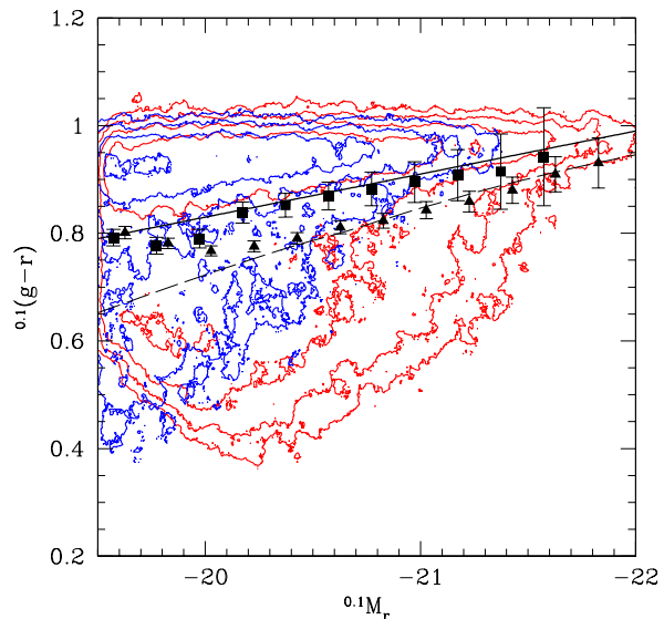
Figure 2. Color-magnitude diagram of M_r < -19.5 volume-limited SDSS catalog constructed from the Y07 group catalog. Contours for central galaxies (with brightest r -band luminosity) and satellite galaxies are red and blue, respectively. The satellite galaxy color-magnitude sequence \langle c|L \rangle_{\text{sat}} of the SS08 model (1) is shown as the thick solid line; the mean satellite galaxy colors at fixed luminosity of the group catalog are shown as the square points, with Poisson errors. The color-magnitude sequence of central galaxies in the model (5) and the group catalog are also shown, by the dashed line and triangle points, respectively. The measured central and satellite colors (squares and triangles) are slightly offset, for clarity.
