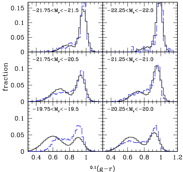
Figure 3. Distributions of g-r color of central galaxies as a function of luminosity. Solid black histograms show the predictions of the model (Skibba & Sheth 2008); Dashed blue histograms show the measurements from the Yang et al. (2007) group catalog.
