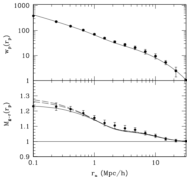
Figure 1. Projected two-point correlation function and g-r color mark correlation function for M_r < -19.5 . Points show SDSS measurement for Petrosian colors, and solid curves show the fiducial model, both taken from Skibba & Sheth (2008). Dashed curves show the range of color mark correlations predicted by the model if color gradients in groups and clusters are included (Hansen et al. 2007).
