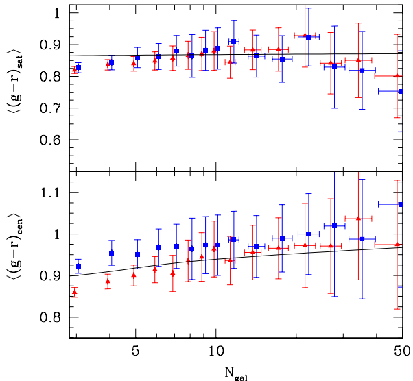
Figure 5. Mean central and satellite g-r colors as a function of group richness, for M_r < -19.9 . Solid curves show the model predictions (using equations 6 and 7), and red triangles and blue squares show the measurements from the B06 and Y07 galaxy group catalogs, respectively. Vertical error bars are the average of the Poisson errors (estimated from the number of groups in each bin) and bootstrap errors (estimated from the variance of 10 times as many pseudo-samples as the number of groups). Horizontal error bars show the N_{\text{gal}} bin widths.
