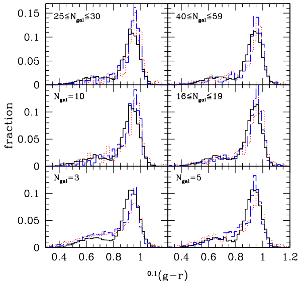
Figure 7. Same as Figure 6, but for satellite galaxies. The three large N_{\text{gal}} bins are chosen to be the same as the 5 th -richest, 3 rd -richest, and richest bins in Figure 5.
