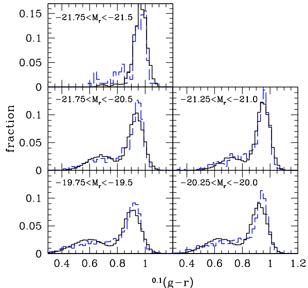
Figure 4. Same as Figure 3, but for satellite galaxies. The brightest luminosity bin is excluded because of poor number statistics.
